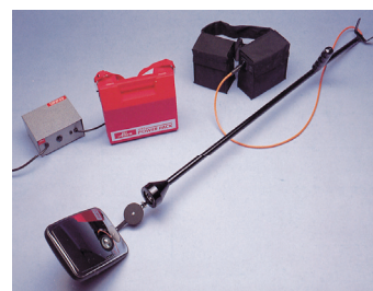
電池燈照明車底檢查鏡 UNDER VEHICLE TROLLEY MIRRORS W/HIGH POWER LAMP
